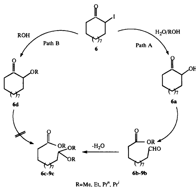
Scheme 2. Photochemical process of \alpha -iodocycloalkanones.
